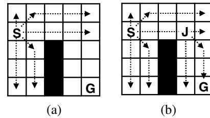
Figure 5: Basic JPS example.
