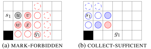
Figure 4: Explaining c_i \geq 6 . Filled nodes are obstacles, red nodes are explored by \text{MARK-FORBIDDEN} , blue nodes explored by \text{COLLECT-SUFFICIENT} . Dashed nodes were pruned due to H .
